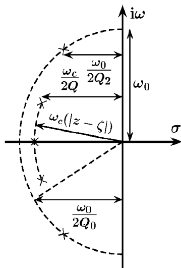
Pole-zero diagram
