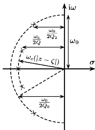
Pole-zero diagram
