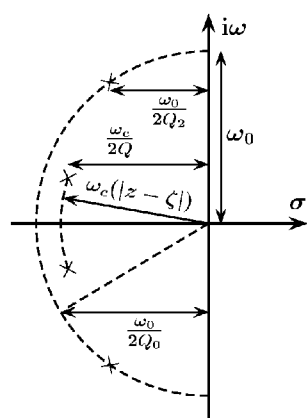
Pole-zero diagram
