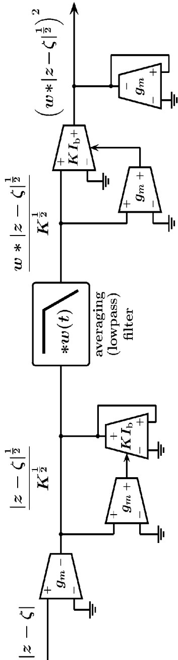
Example of windowed Squared Mean Root (SMR) circuit
