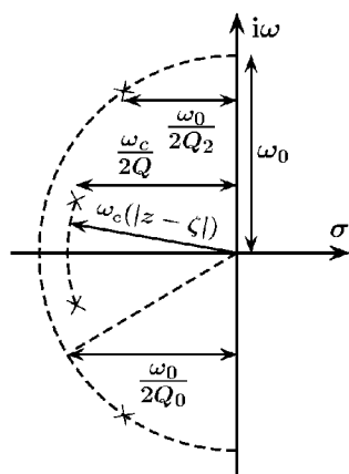
Pole-zero diagram
