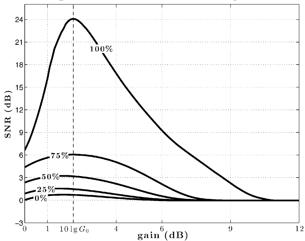
SNR vs gain for different fractions of impulsive noise
